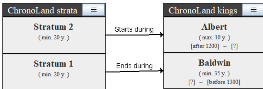
Figure 21. Modelling the ChronoLand data with ChronoLog (showing inputs only).
