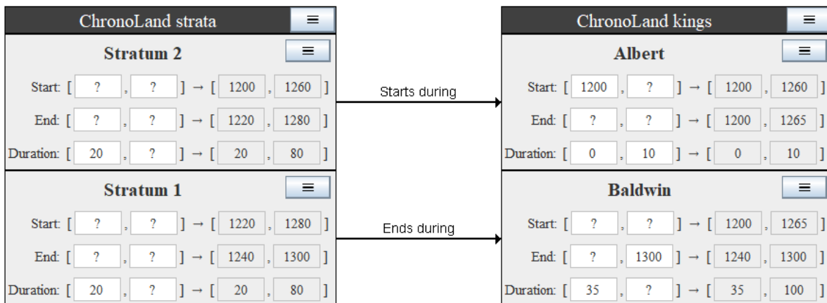
Figure 23. Modelling the ChronoLand data with ChronoLog ("Full view")
