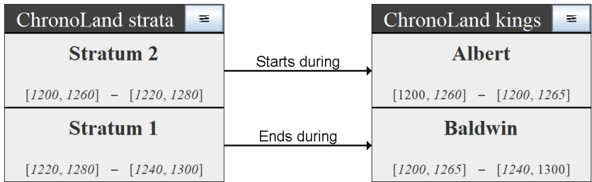
(b) Concise view (no durations)
