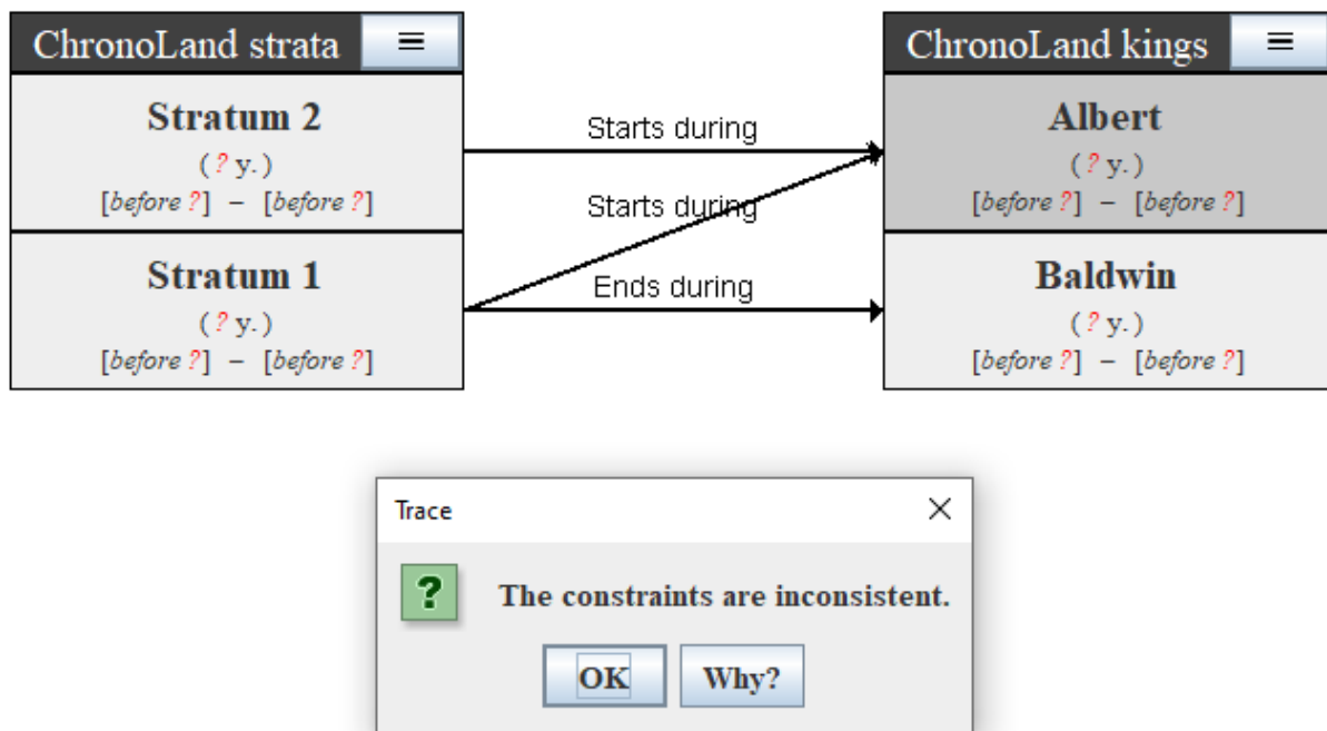
Figure 28. Result of adding the synchronism "Stratum 1 starts during Albert" to the model. ChronoLog detects an inconsistency, implying that stratum 1 was built during Baldwin's reign.
