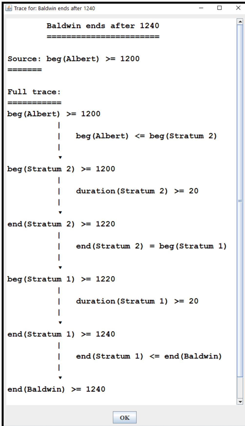
Figure 24. A justification of the computed 1240 lower bound for the end of Baldwin's reign, as obtained by Chronolog (by clicking on the "1240" button).
