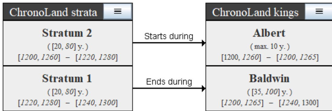
Figure 22. Modelling the ChronoLand data with ChronoLog (showing all data)
