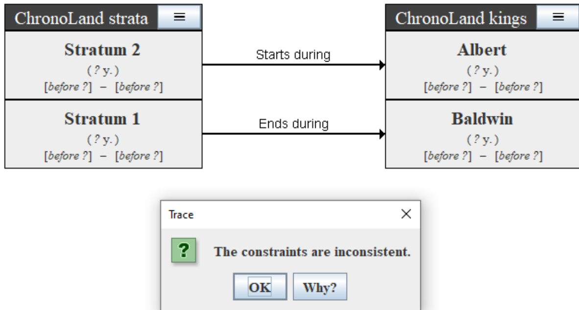
Figure 25. Changing the duration bounds of Baldwin to maximum 25 years yields an inconsistency result.
